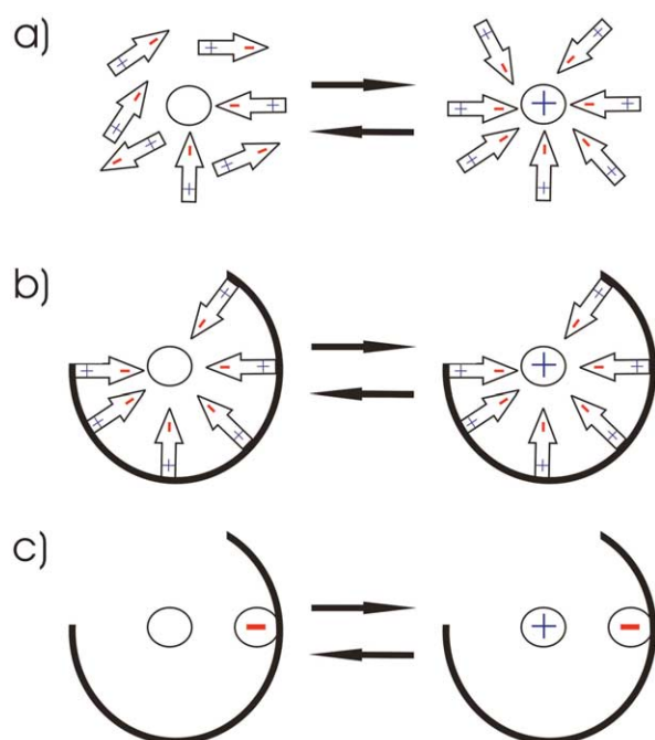
Fig. 1. Three different charge-compensating scenarios (modified from [11]). a: The charge is placed in a medium with a high dielectric constant. b: The charge is stabilized by a set of prearranged dipoles. c: The charge is stabilized by a counter ion.
